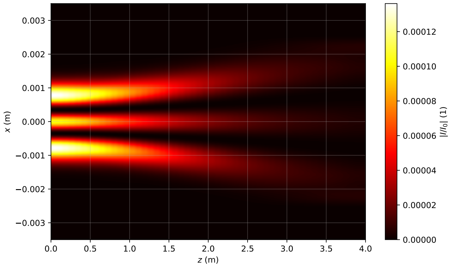
Intensity profile I(x, y = 0, z)/I_0 , P_{in}=0.5P_{cr} , artificial time
